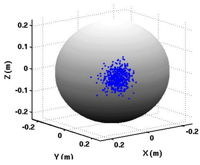
Figure 7: Impact Locations on Surface of 1999RQ36
