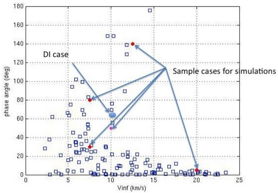
Figure 3: Phase vs. V_{\infty} for Candidate Mission Set (data from [2])
