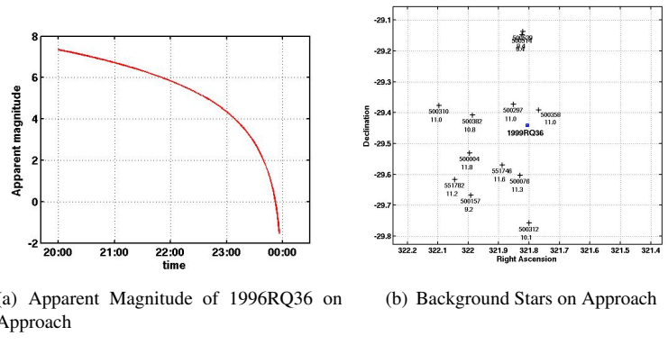
Figure 6: Apparent Magnitudes of 1996RQ36 and Background Stars During Terminal Guidance Phase
