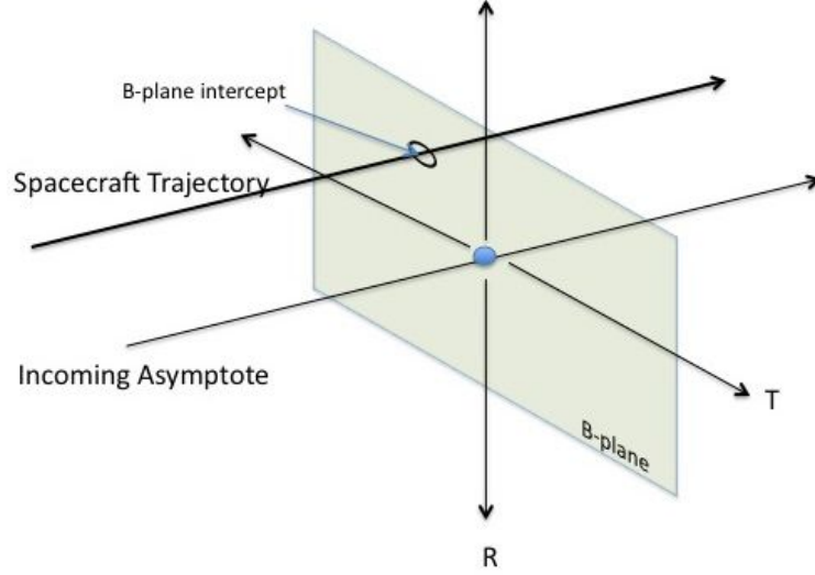
Figure 1: B-plane coordinate system
