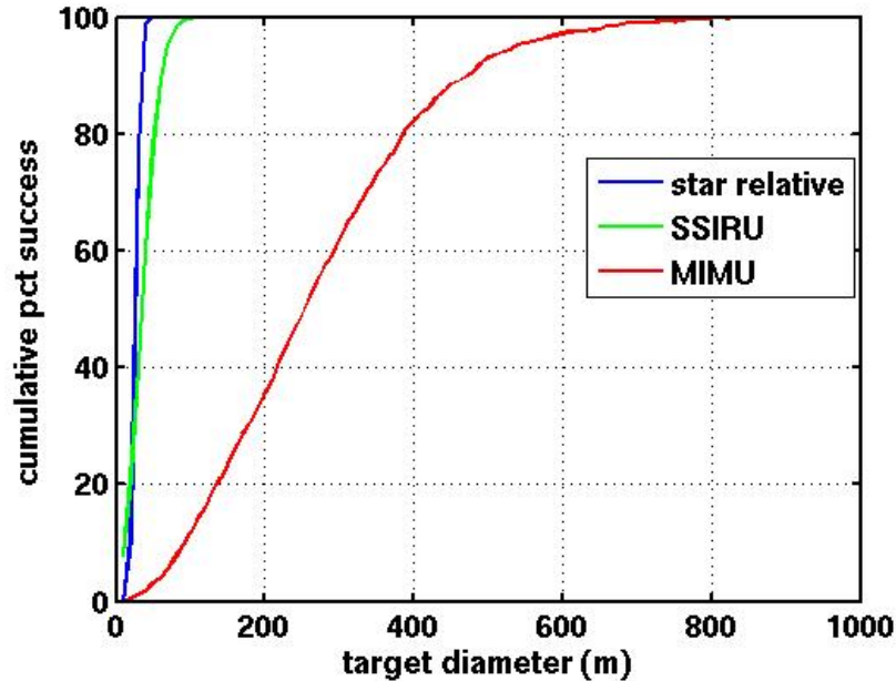
Figure 4: Cumulative probability as a function of miss distance for three attitude modes
