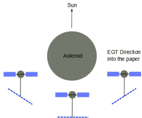
Figure 18: Multiple EGTs on Solar Sails.
